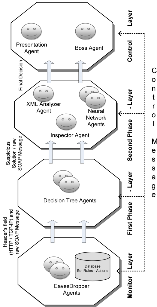
Fig.1. Design of the multi-agent architecture proposed
